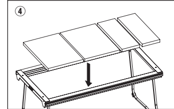
Flip the entire table unit back from the upside-down position and install it. According to your preferred layout, place tabletops and/or IGT unit items on the top.
