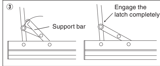
Engage the support bar shown above. (4 locations)
